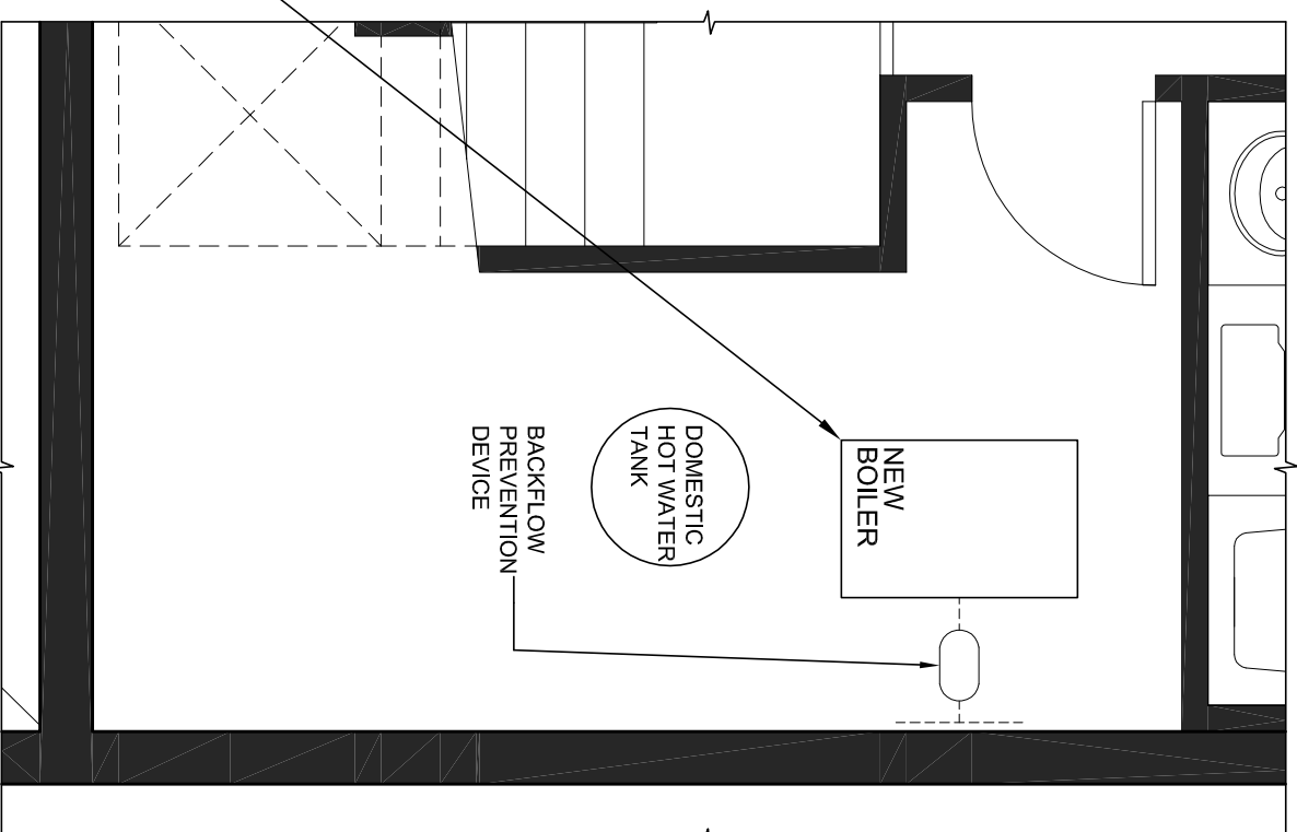
NEW BOILER LAYOUT
