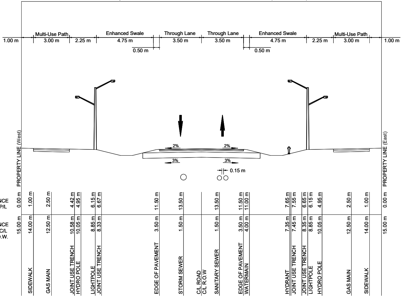
Clarkway Drive - Recommended Cross-Section, Mid-Block (30 m ROW)
