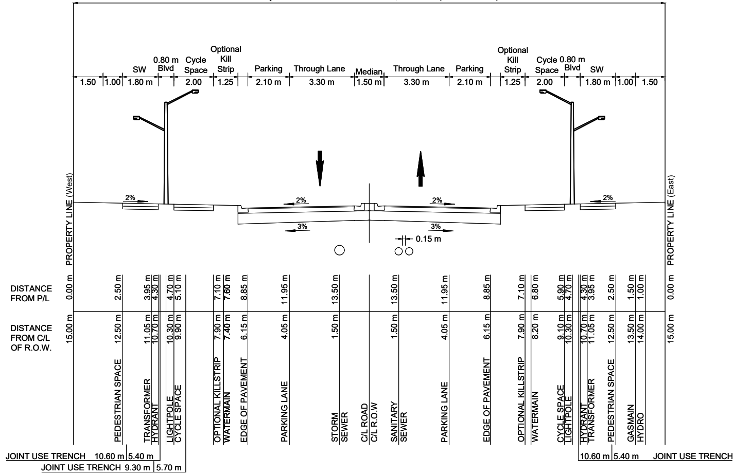
Clarkway Drive - Alternative Cross-Section, Mid-Block (30m ROW min)
