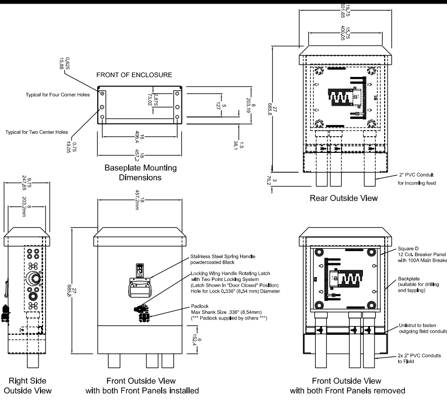
SLS Un-metered Pedestal (Typical Layout) PART NO. SLS1-8-40(100)
