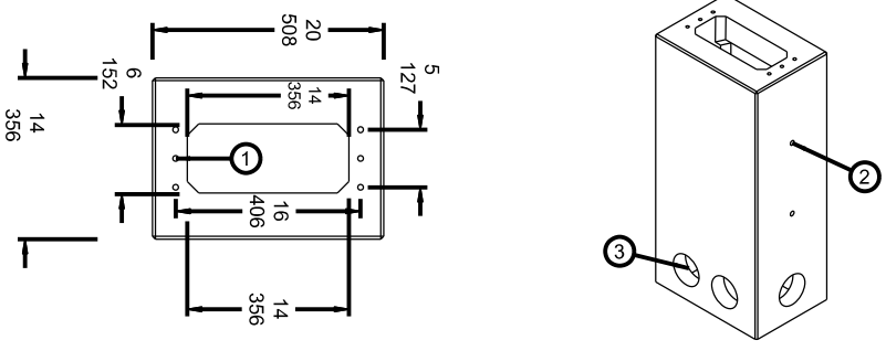
SLS Un-metered Pedestal (Typical Layout) PART NO. SLS1-8-40(100)
