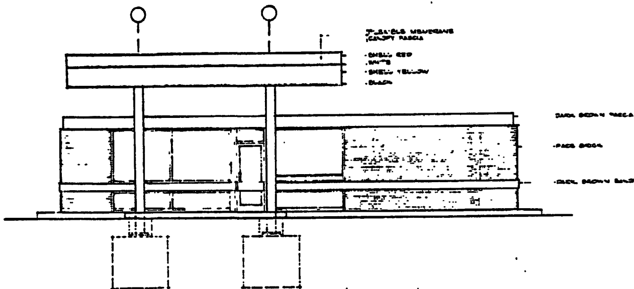
EAST ELEVATION
