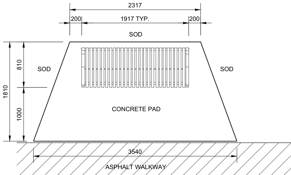
CONCRETE BENCH PAD: PLAN
