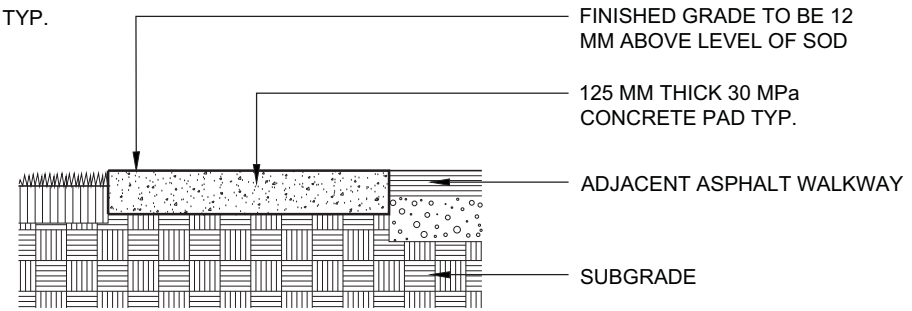
CONCRETE BENCH PAD: SIDE SECTION
