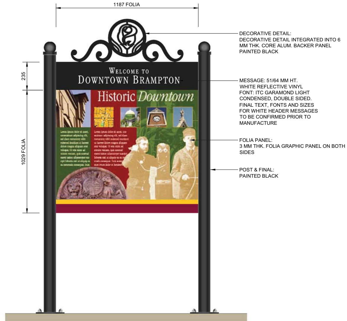
FRONT ELEVATION
