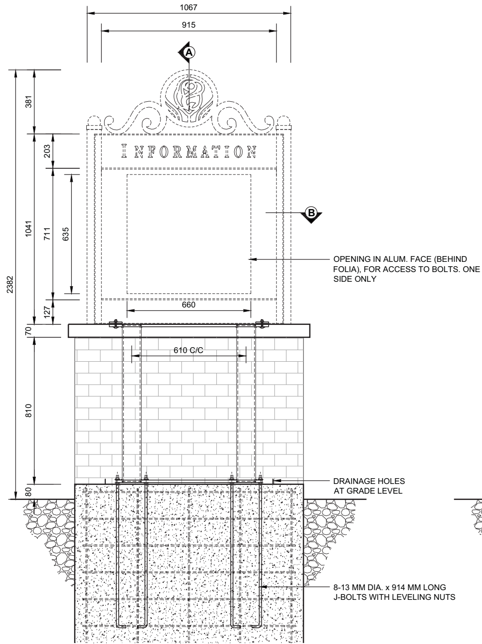
FRONT ELEVATION
