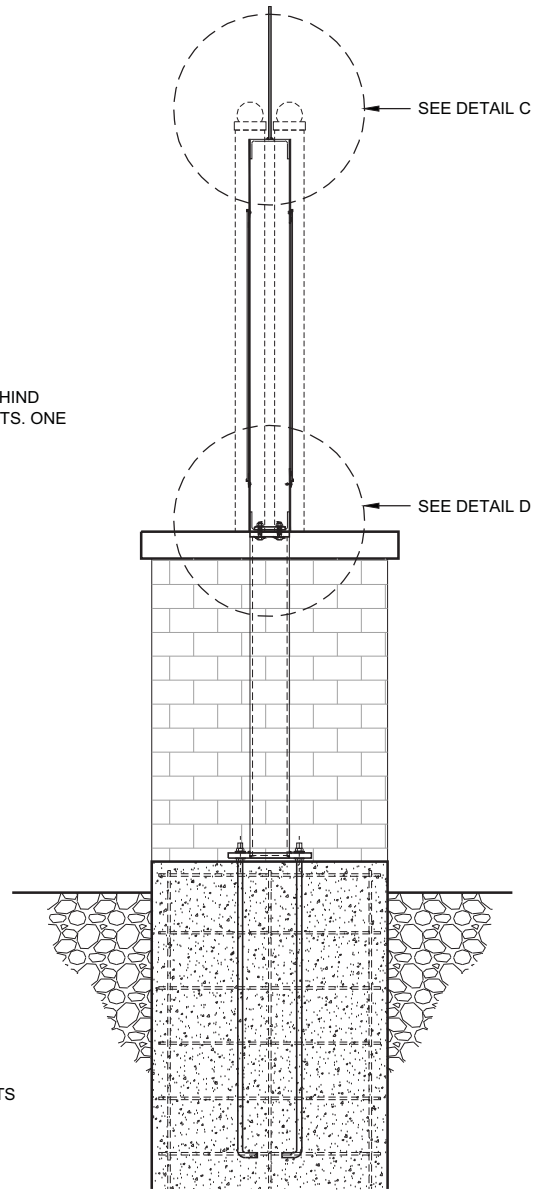
SECTION A
