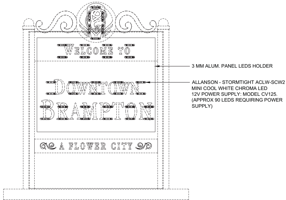
LED LAYOUT
