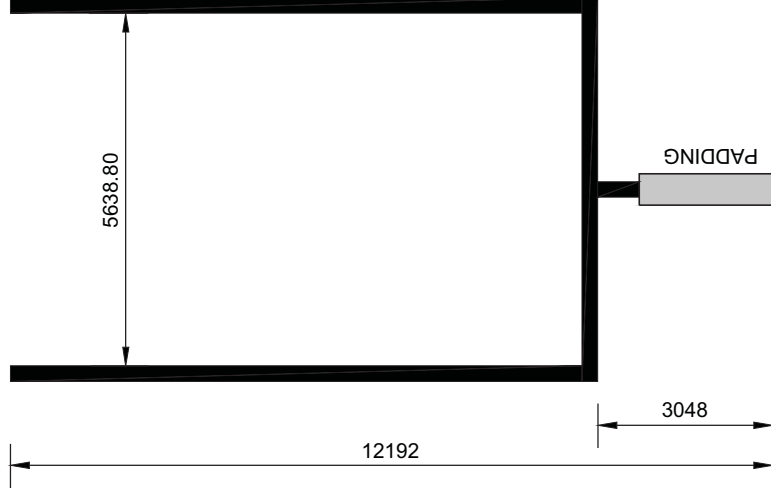
GOAL POST DETAIL
