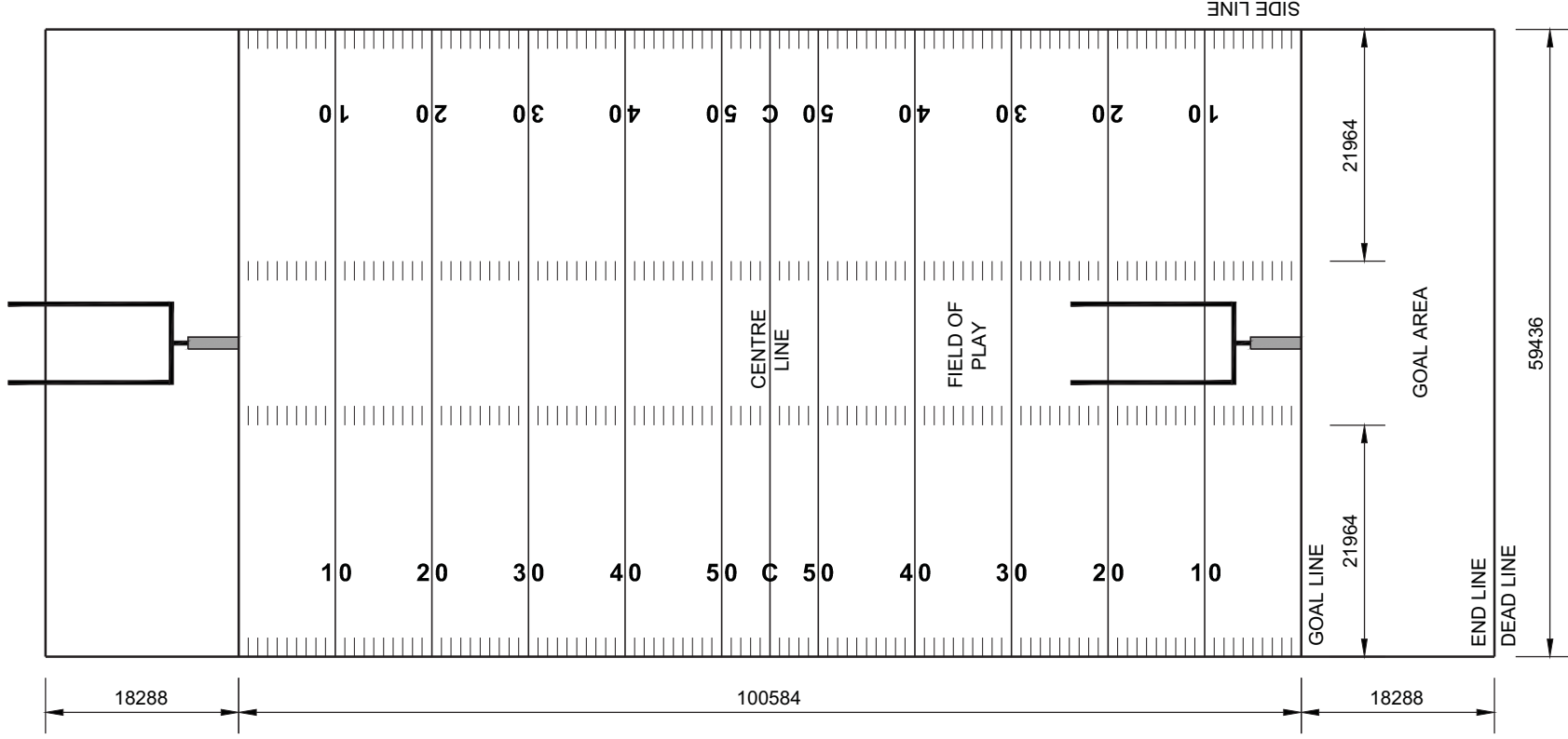
FIELD LAYOUT
