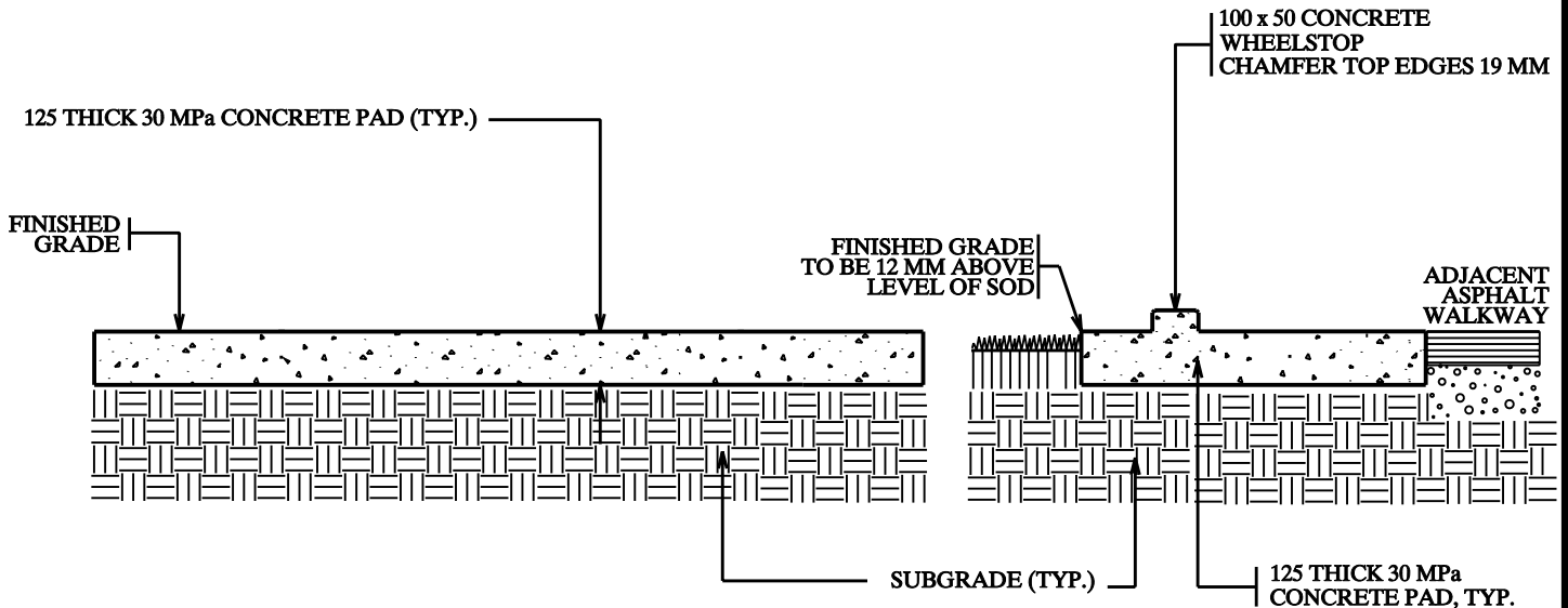
CONCRETE BENCH PAD, FRONT SECTION
