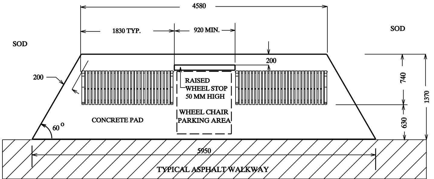
CONCRETE BENCH PAD, PLAN VIEW
