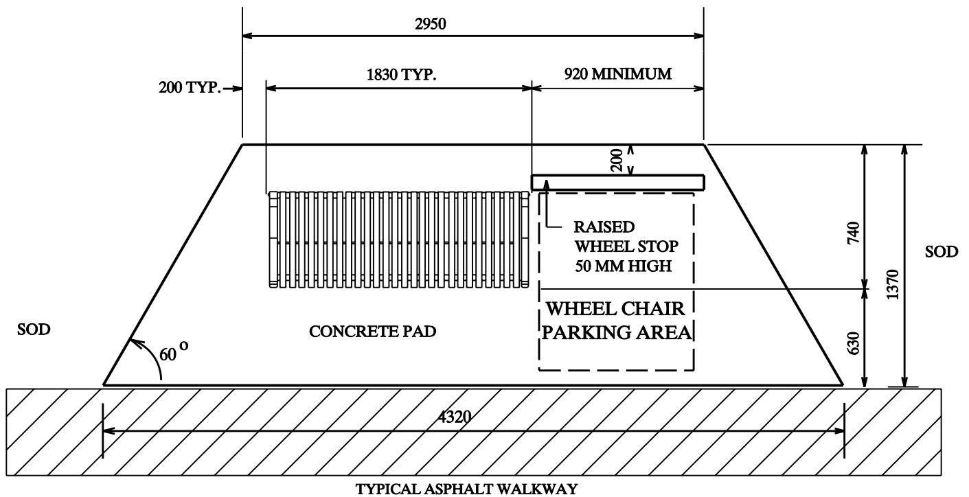
CONCRETE BENCH PAD, PLAN VIEW
