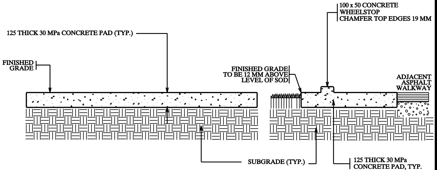
CONCRETE BENCH PAD, SIDE SECTION
