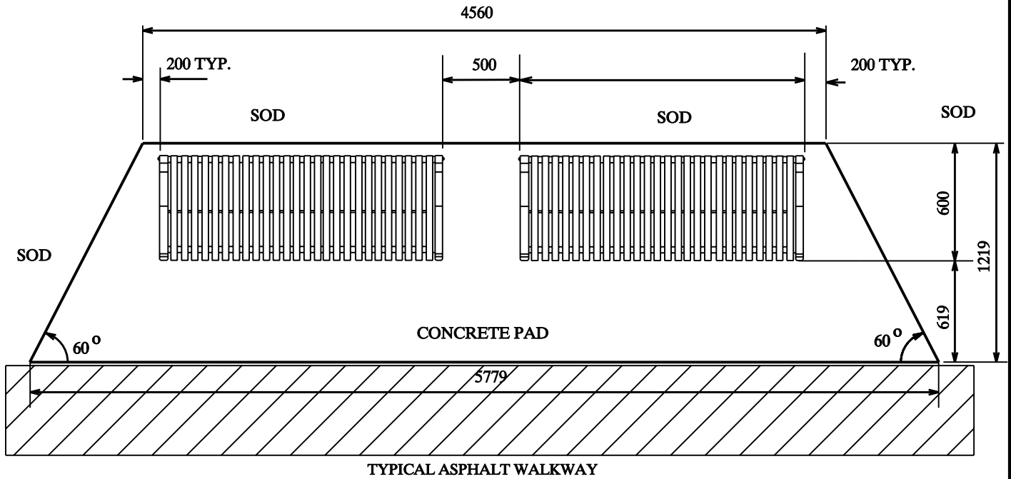
CONCRETE BENCH PAD, PLAN VIEW (2 BENCHES)
