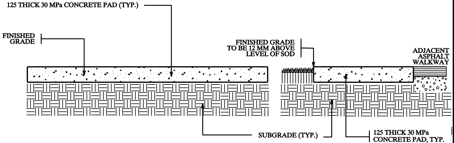
CONCRETE BENCH PAD, FRONT SECTION
