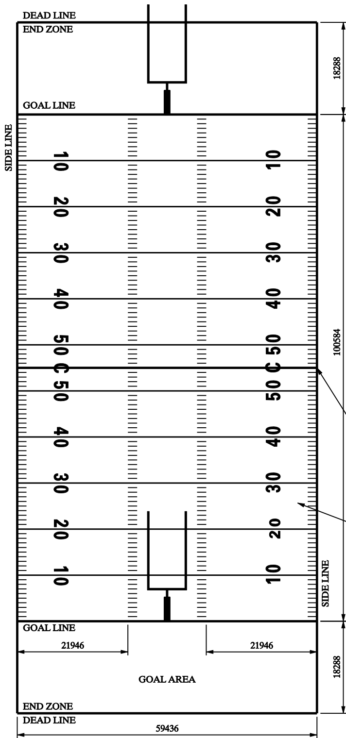
FIELD LAYOUT
