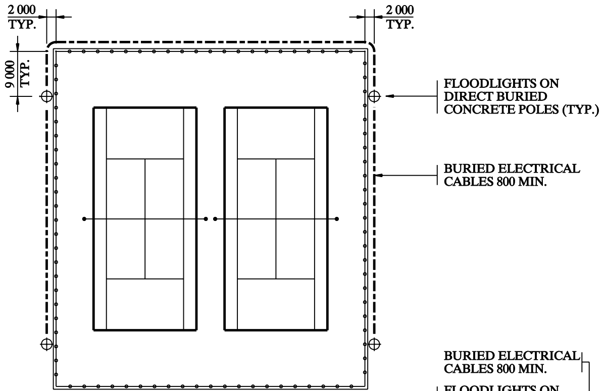
2 - COURT LIGHTING LAYOUT
