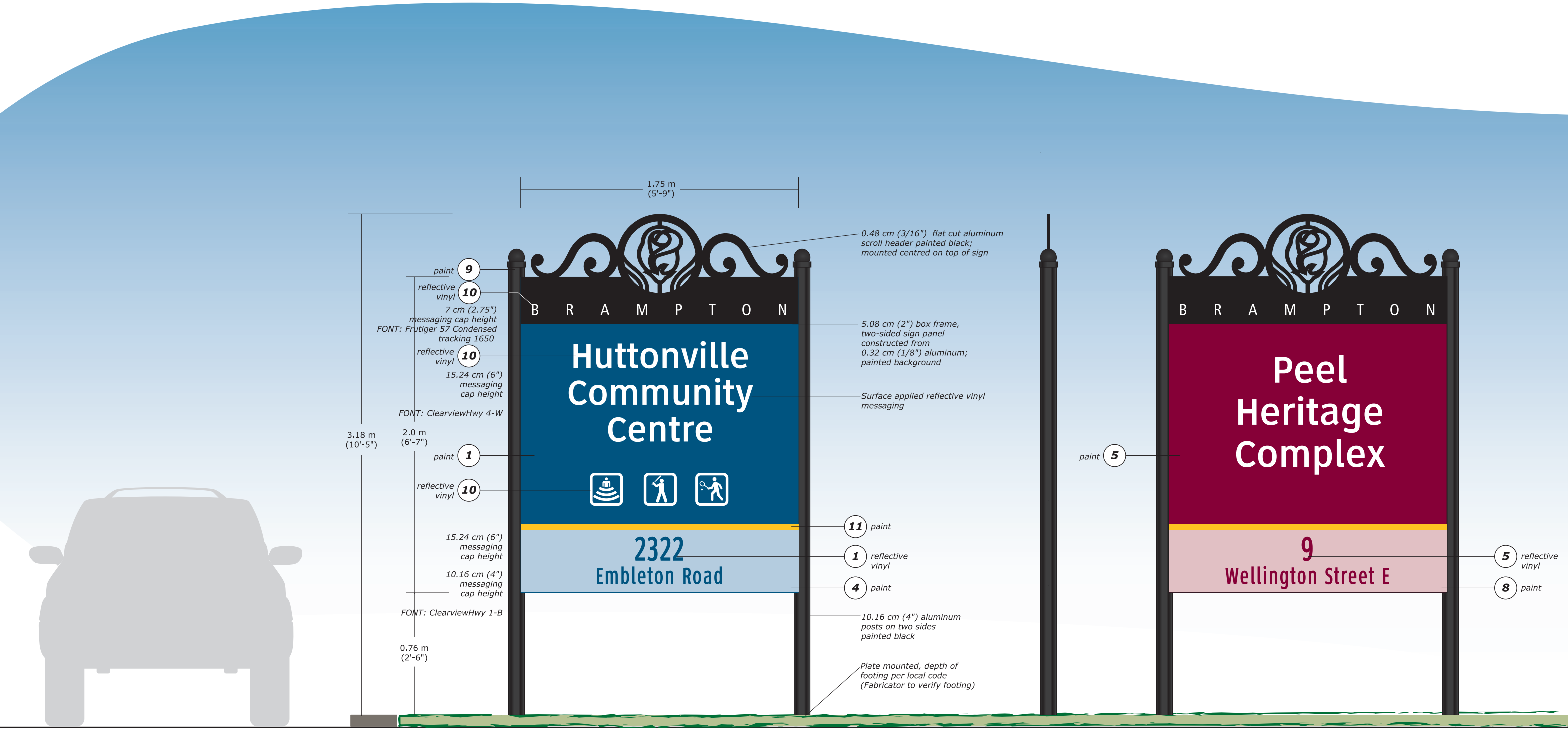
Front View (Back View is identical with reflected scroll header) (Two-Sided Sign)
