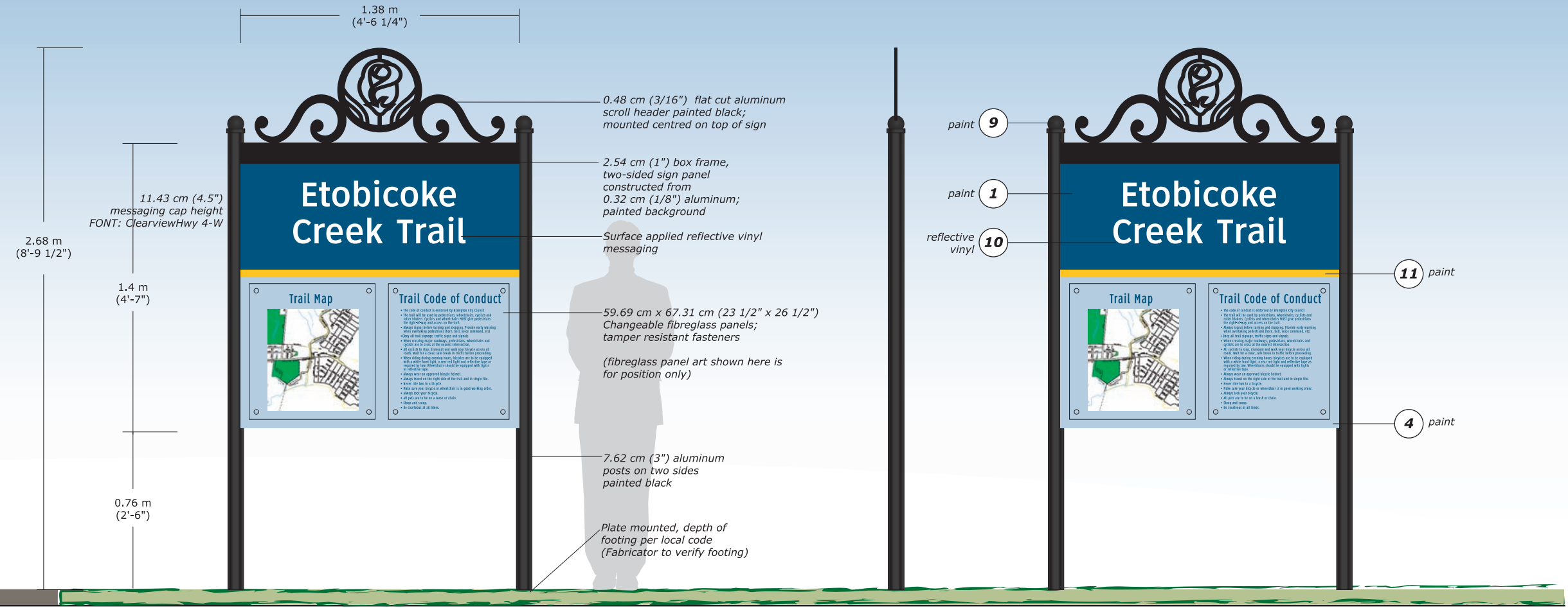
Front View (Two-Sided Sign)
