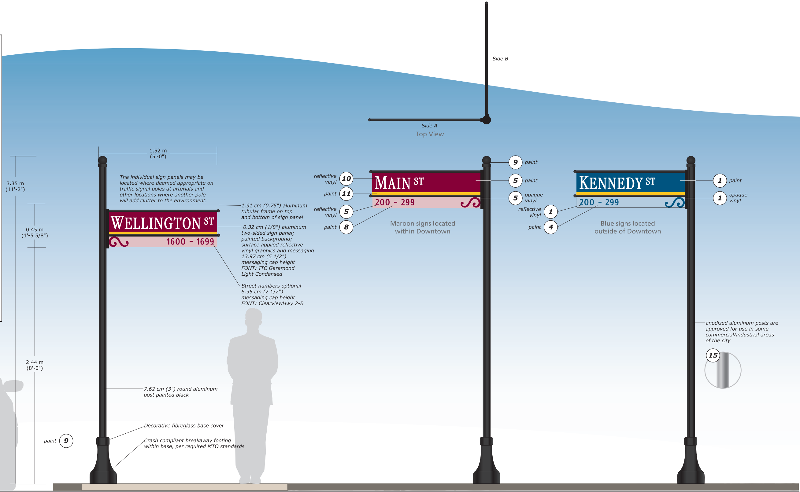
Side A View (Two-Sided Sign)
