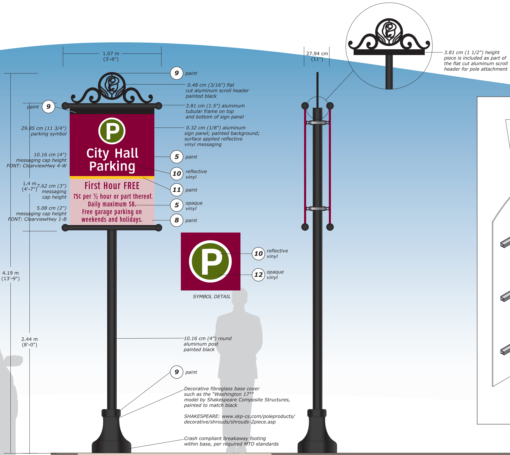
Front View (Back View is identical with reflected scroll header) (Two-Sided Sign)
