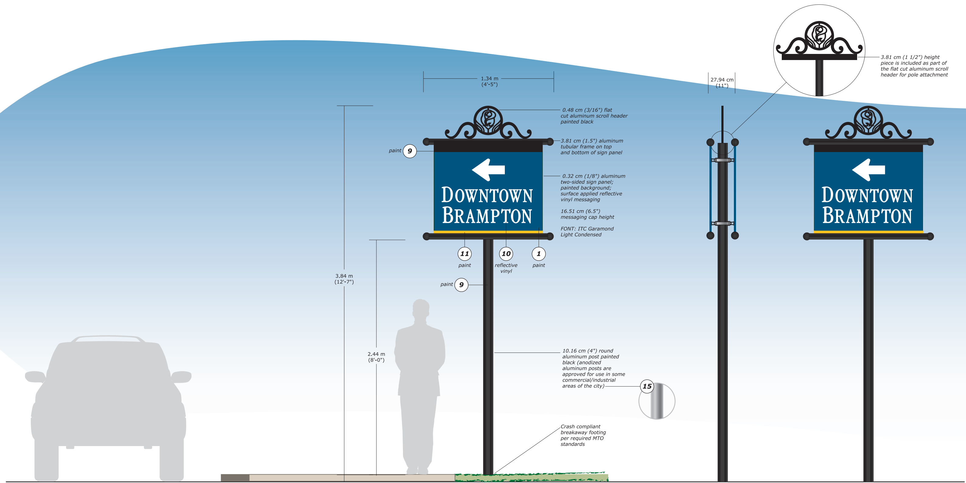
Front View (Two-Sided Sign)
