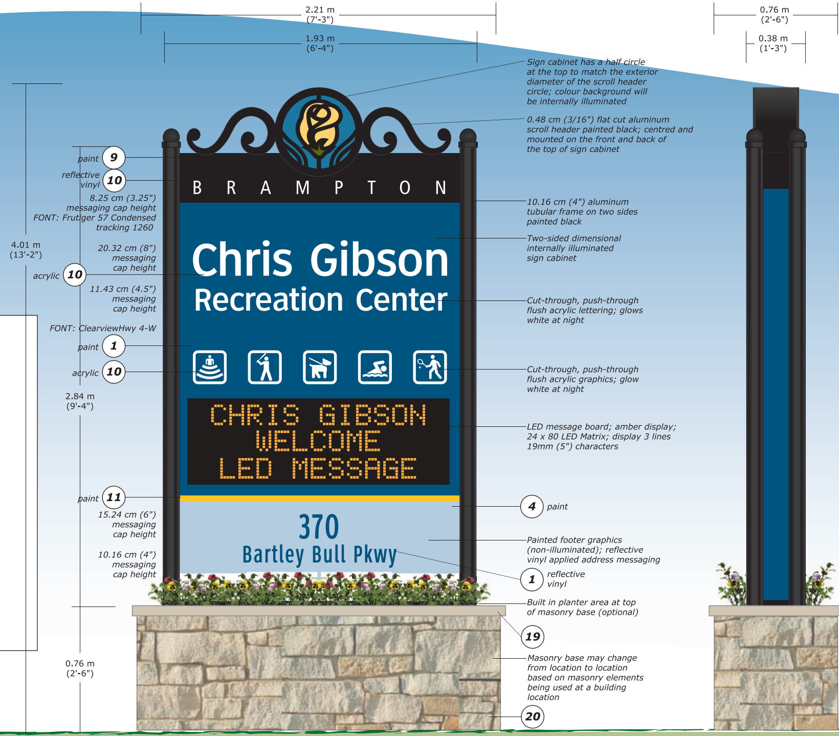
Front & Back Views (Two-Sided Sign)
