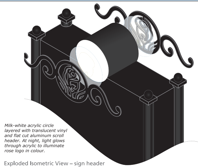
Exploded Isometric View – sign header
